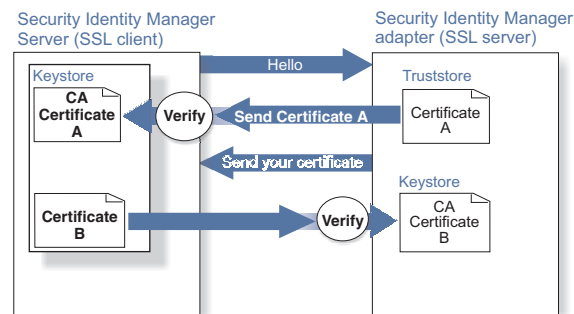
Figure 2. Two-way SSL authentication (client authentication)
